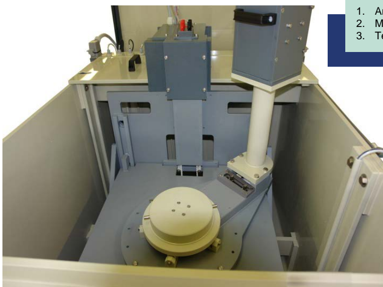
Lifting/lowering table with mounted rotation unit and bayonet catch fitted into electro-plating tank.
